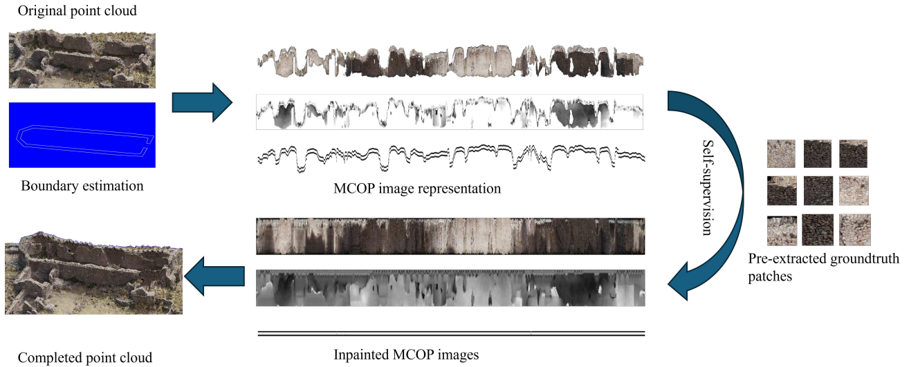
Figure 3. General pipeline of our MCOP based point cloud completion method. The input point cloud is first projected onto a 2D image with 5 channels (RGBD + rotation) using our MCOP representation. During training, a random sampling function f_\theta is applied on the MCOP image to extract a group of local windows, which are trained against mostly complete local patches extracted from the dataset of all structures in an adversarial way. For inference, the MCOP image and an outline of the desired shape (e.g., wall height) is passed to our inpainting network adapted from [35]. The final completed point cloud is obtained by remapping the inpainted MCOP image back into 3D.
