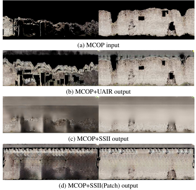
Figure 10. Demonstration of the necessity of applying patch based self supervision for inpainting our MCOP images.
