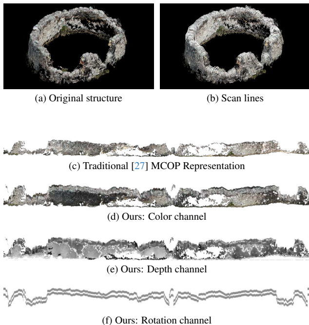
Figure 4. MCOP [27] representation. For (a), we sample along a circular path while MCOP camera captures scan lines perpendicular to the path (b). Instead of the traditional MCOP image (c), we capture a 5 channel image (d, e, f).
