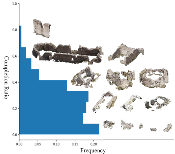
Figure 5. Histogram of random point cloud samples from the Mawchu Llacta dataset, with high completion ratios at the top to low-completion ratios at the bottom.
