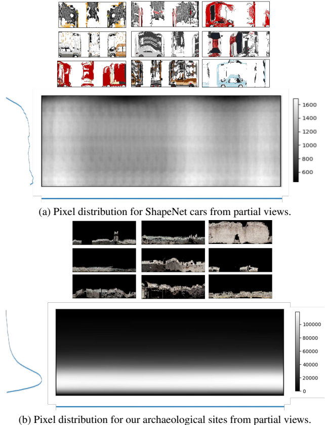
Figure 2. Comparison of distribution of available points for incomplete point clouds suffering from occlusion/partial view and missing surfaces. The distributions are quite different and that of our outdoor sites is clearly vertically unbalanced.
