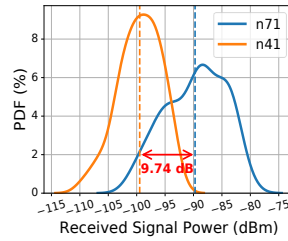
Figure 28: FDD-TDD CA expands 5G coverage. (a) Low-band (n71) receives higher signal power under challenge scenarios. (b) Lock/unlock the use of FDD low-band (n71).
