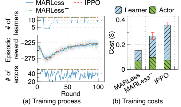
Figure 12: MARLess reduces costs by combining dynamic learner sharing and actor scaling with serverless computing.
