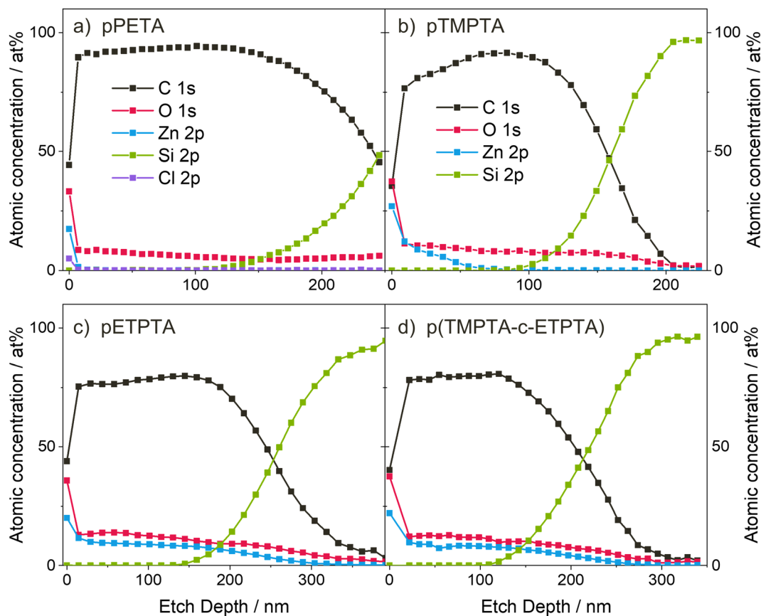
Fig. 5 XPS depth profiles of (a) pPETA after 5 minutes UV exposure, and (b) pTMPTA, (c) pETPTA and (d) p(TMPTA-c-ETPTA) after 10 minutes UV exposure and VPI with a 15-hour DEZ hold at 120 °C.
