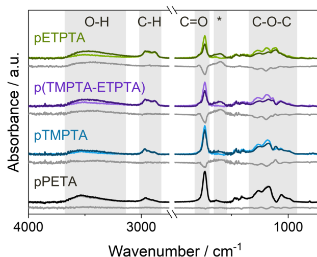
Fig. 4 FTIR spectra of crosslinked acrylate films before (light color) and after (dark color) VPI with a 15-hour DEZ hold at 120^\circ \text{C} . The difference spectra are shown as gray lines. Relevant absorption bands are highlighted in gray. *marks a new peak that appears upon reaction with DEZ. pPETA was UV-polymerized for 5 min, pTMPTA, p(TMPTA-ETPTA) and pETPTA for 10 min.
