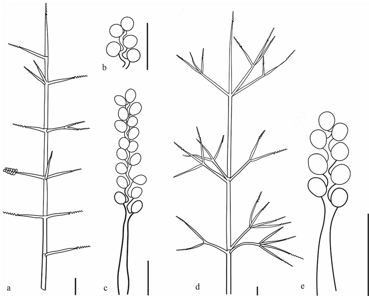
Fig. 31 Tritirachium sp. a–c T. dependens . d, e T. album . Scale bars: a–e = 10 \mu m (redrawn from Limber 1940)
