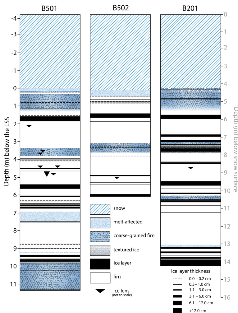
Figure 2. Stratigraphy of the three firn cores drilled at Eclipse Icefield in 2023. The position of the LSS 0 m ark on the left-hand depth scale is the mean LSS depth (4.27 m).
