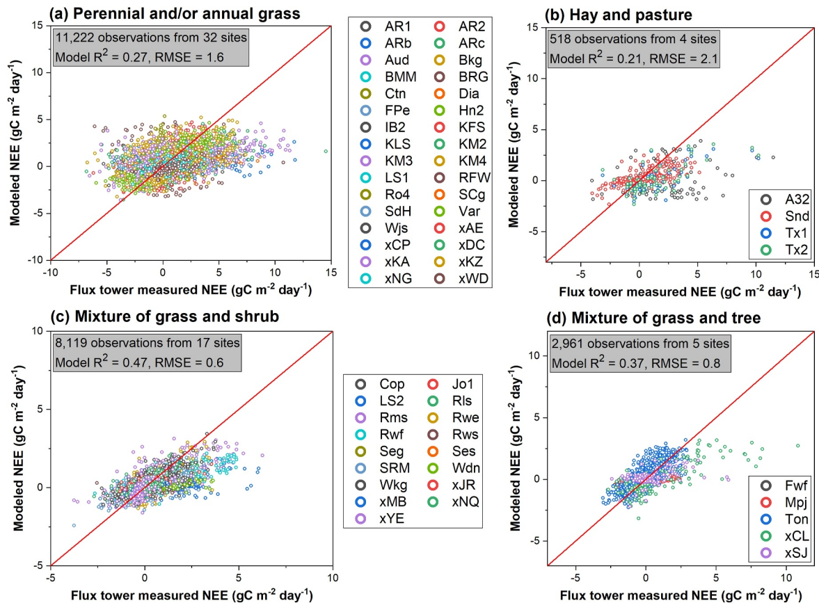
Figure 5. Model fit for net ecosystem exchange of CO 2 (NEE) represented by the coefficient of determination (R 2 ) and root mean square error (RMSE, C m -2 day -1 ) for different vegetation classes including (a) perennial and/or annual grass, (b) managed hay and pasture, (c) mixture of grass and shrub, and (d) mixture of grass and tree classes. Positive NEE sign denotes ecosystem carbon sink activity. Different colors represent different study sites.
