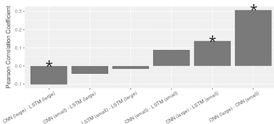
Fig. 14 Agreement between model variants on sub-sequence prediction. From left to right: r(798) = -0.1018, p < .05 ; r(798) = -.0442, p < .1 ; r(798) = -.0155, p < .1 ; r(798) = .0892, p < .1 ; r(798) = .1369, p < .01 ; r(798) = .3070, p .001
