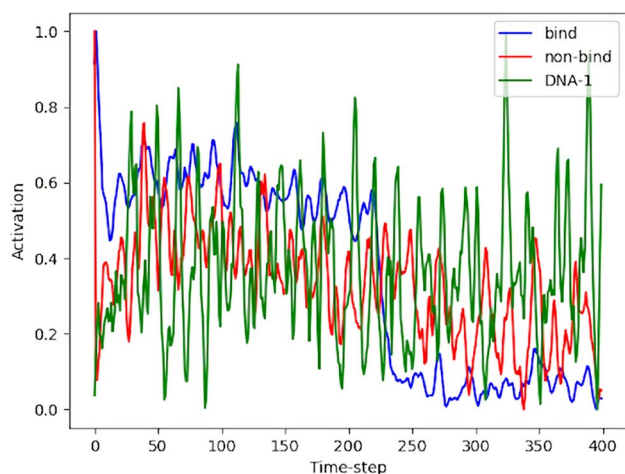
Fig. 7 Non-binding, binding, and DNA-1 activations from LSTM hidden cell standardized between 0 and 1
