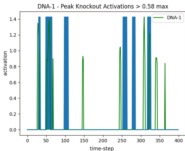
Fig. 11 Peak knockout occluded DNA-1 activations processed according to equation on for peaks at 58% threshold, r(798) = 0.257 , p .01
