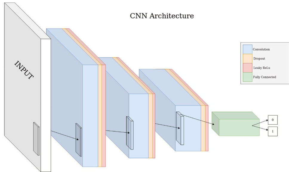
Fig. 4 CNN model architecture
