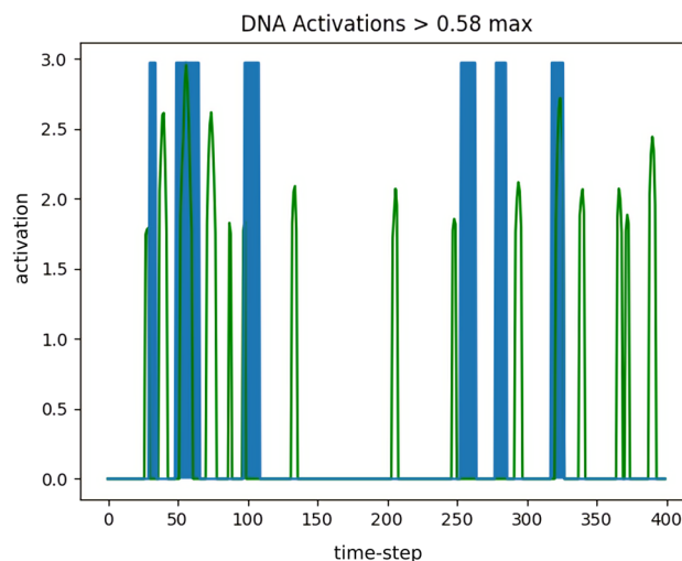
Fig. 9 DNA-1 activations processed according to equation one for peaks at 58% threshold, r(798) = 0.143 , p = .01
