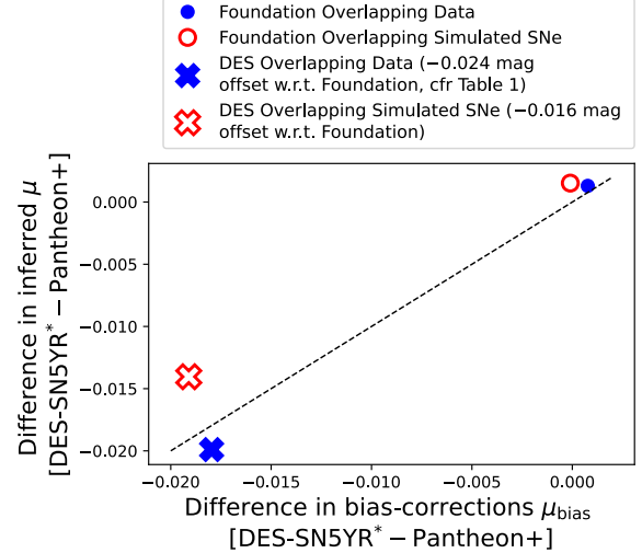
Figure 4. For the DES and Foundation sub-samples of overlapping SNe between DES-SN5YR* and Pantheon+, we compare the difference in bias corrections \mu_{bias} with the difference in distance moduli, \mu . Differences relative to the Foundation (DES) sub-sample of overlapping data are marked with circles (crosses). Filled blue symbols correspond to differences in the real data, while empty red symbols correspond to differences estimated from simulations. Instead of using the original DES-SN5YR distance moduli, we use distances from a re-analysis using the Pantheon+ modelling as described in Section 4. For this reason, differences in measured distance moduli from the data are -0.024 (and not -0.042 , see Table 1). To avoid confusion with different M_0 , we subtract 0.04 mag from all the DES-SN5YR bias-corrections. Using simulations, we quantify the expected differences in \mu between the DES sub-samples in Pantheon+ and DES-SN5YR to be -0.016 .
