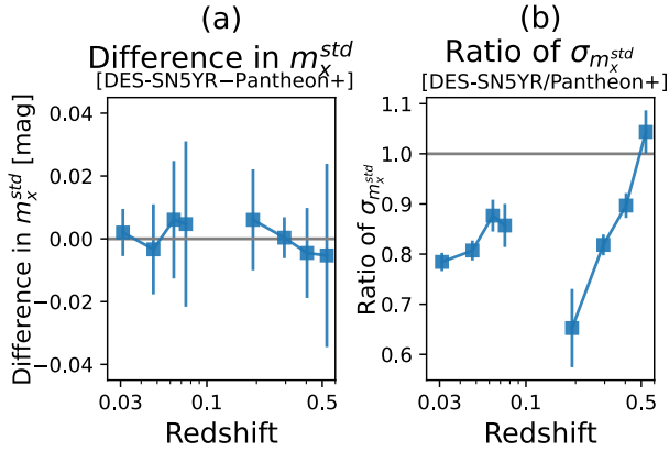
Figure 1. Left panel: Median m_x^{\text{std}} difference vs. redshift (and error on the median) for common SNe in DES-SN5YR and Pantheon+. Across all redshifts, differences in m_x^{\text{std}} are consistent with zero. Right panel: ratio of m_x^{\text{std}} uncertainties between DES-SN5YR and Pantheon+. For a more direct comparison, we measure m_x^{\text{std}} and its uncertainty using the same nuisance parameters for both DES-SN5YR and Pantheon+: \alpha = 0.15 , \beta = 3.1 , \gamma = 0 .
