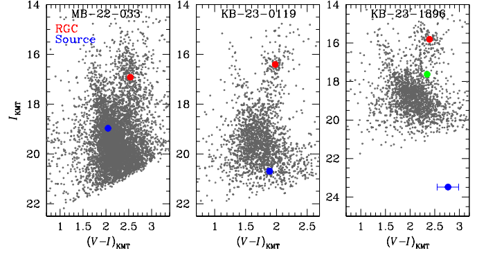
Fig. 8. Locations of source stars (filled blue dots) in the instrumental color-magnitude diagrams. The red dot in each panel indicates the centroid of red giant clump (RGC).
