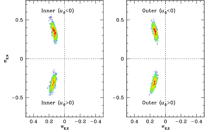
Fig. 2. Scatter plots of points in the MCMC chain on the (\pi_{E,E}, \pi_{E,N}) parameter plane. Colors are chosen to present points with \leq 1\sigma (red), \leq 2\sigma (yellow), \leq 3\sigma (green), \leq 4\sigma (cyan), and \leq 5\sigma (blue).
