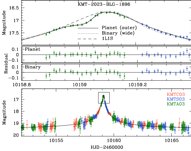
Fig. 6. Light curve of KMT-2023-BLG-1896.
