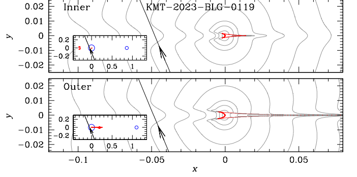
Fig. 5. Configurations of the lens system for the inner and outer solutions of KMT-2023-BLG-0119. The inset in each panel offers a zoomed-out view. In the inset, blue empty circles mark the positions of the lens components: a small circle for the planet and a large circle for the host.
