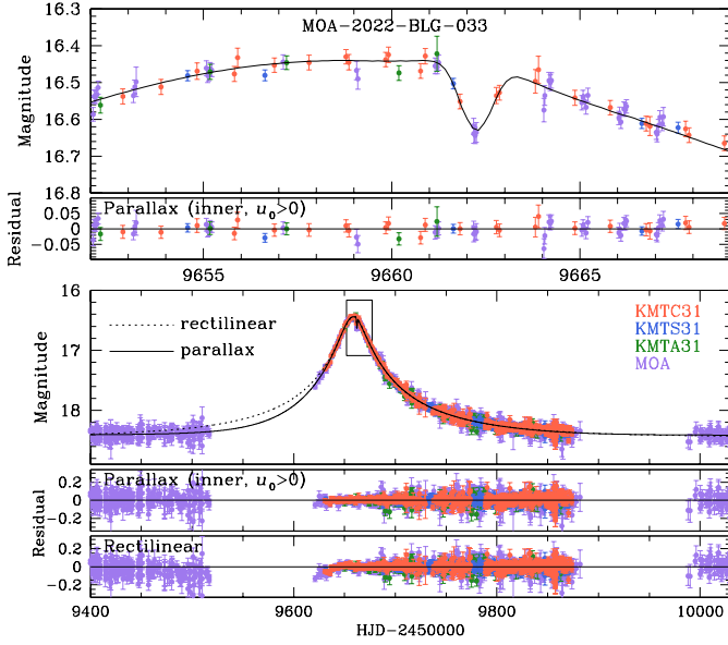
Fig. 1. Light curve the lensing event MOA-2022-BLG-033 and the model curve. The lower panel offers a comprehensive view of the event, while the upper panel provides a close-up view of the anomaly (the region enclosed by a box in the lower panels). The colors of the data points correspond to the telescopes listed in the legend. The bottom two panels show the residuals from the models with and without considering microlens-parallax effects.
