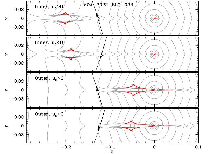
Fig. 3. Lens-system configurations for the four degenerate solutions of MOA-2022-BLG-033. In each panel, the red figure represents the caustic, and the arrowed curve indicates the source trajectory. The grey curves surrounding the caustic represent equi-magnification contours. The coordinates are centered on the position of the primary lens, and the lengths are scaled to the Einstein radius.
