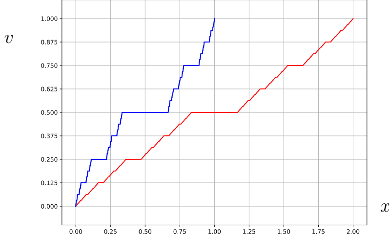
Figure 2: Cantor expansion wave: v = c(z) vs. x = z + tc(z) at t = 0 and 1.
