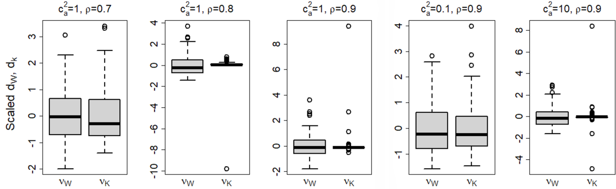
Figure 8: Box plots of the scaled distance obtained from 100 bootstrap sample sets. The queuing capacity is set to 1,000. The spreads in the Kingman distance are smaller than in the Wasserstein distance.
