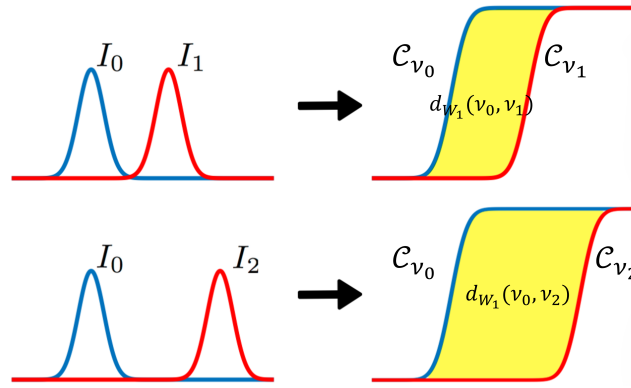
Figure 2: The 1-Wasserstein distances d_{W_1}(\nu_0, \nu_1) and d_{W_1}(\nu_0, \nu_2) in 1-D computes the areas between the CDFs \mathcal{C}_{\nu_0} and \mathcal{C}_{\nu_1} , and \mathcal{C}_{\nu_0} and \mathcal{C}_{\nu_2} , respectively. As the distance between the distributions increases, so does d_{W_1} .
