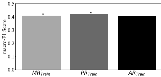
(a) Macro-F1 scores on MR set.
