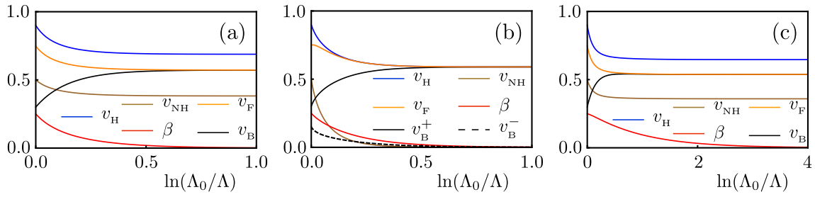
Figure 3: Renormalization group flows for various velocity (fermionic and bosonic) and birefringent ( \beta ) parameters close to the (a) CI, (b) CII, and (c) CIII mass generations, discussed in Sec. 4.1, Sec. 4.2, and Sec. 4.3, respectively, for N_f = 1 , where N_f is the number of four-component fermion species. In all these cases \beta \rightarrow 0 in the deep infrared or quantum critical regime, indicating that four-component spin-3/2 Dirac fermions decompose into two copies of two-component spin-1/2 Dirac fermions therein, where they possess a unique terminal Fermi velocity, which is equal to the terminal bosonic velocity, thereby always yielding an emergent Yukawa-Lorentz symmetry. In (a) and (c), we find v_F = v_B with nontrivial v_H and v_{NH} (non-Hermitian Yukawa-Lorentz symmetry). By contrast, in (b) v_H = v_B = v_B^+ = (v_{B_x} + v_{B_y})/2 while v_{NH} \rightarrow 0 (conventional or Hermitian Yukawa-Lorentz symmetry), where v_{B_x} ( v_{B_y} ) is the component of the bosonic velocity in the x ( y ) direction. Near the CII mass generation the rotational symmetry gets broken at intermediate scales as v_B^- = (v_{B_x} - v_{B_y})/2 is finite therein, which however gets recovered in the quantum critical regime where v_B^- \rightarrow 0 . Here, \Lambda_0 ( \Lambda ) is the bare (running) cutoff and \ln(\Lambda_0/\Lambda) \equiv \ell with \ell as the logarithm of the renormalization group scale. Throughout, we set v_H^0 > v_{NH}^0 , where the quantities with the superscript ‘0’ indicate their bare values, such that v_F^0 = \sqrt{[v_H^0]^2 - [v_{NH}^0]^2} is always real, yielding real eigenvalues of the non-Hermitian birefringent Dirac operators. Here, we showcase emergent Yukawa-Lorentz symmetry when v_F^0 > v_{B_x}^0 . We arrive at qualitatively similar conclusions for v_F^0 < v_{B_x}^0 as well (not shown explicitly).
