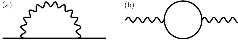
Figure 2: Leading-order (one-loop) self-energy diagrams for (a) non-Hermitian spin-3/2 birefringent Dirac fermions (solid lines) and (b) scalar bosonic order-parameter fields (wavy lines). The interaction vertex corresponds to the Yukawa interaction between these two degrees of freedom.
