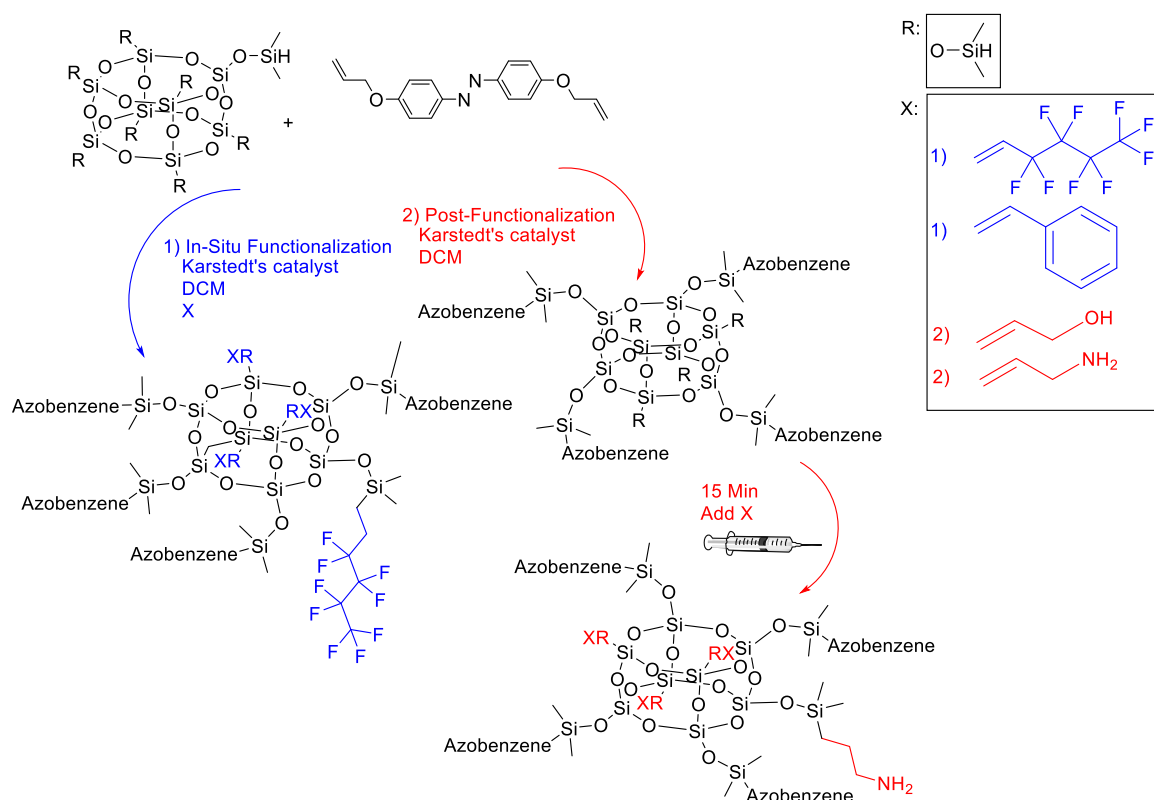
Figure 3. Formation of functionalized gels using in-situ (blue) and post (red) functionalization methods.
