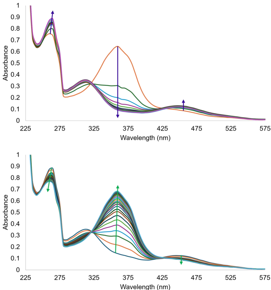
Figure 5. UV-Vis Spectra of the 1-2 Q_8M_8^H – 4,4'-allyloxyazobenzene nonafluoro functional gel. Trans to Cis transition of the azo-crosslinker occurring over 105 seconds of 365nm UV light exposure is shown on top. Conversion from the cis form to the trans happens within 245 seconds of exposure to a 515nm light (bottom). The direction of each transition is shown with arrows.
