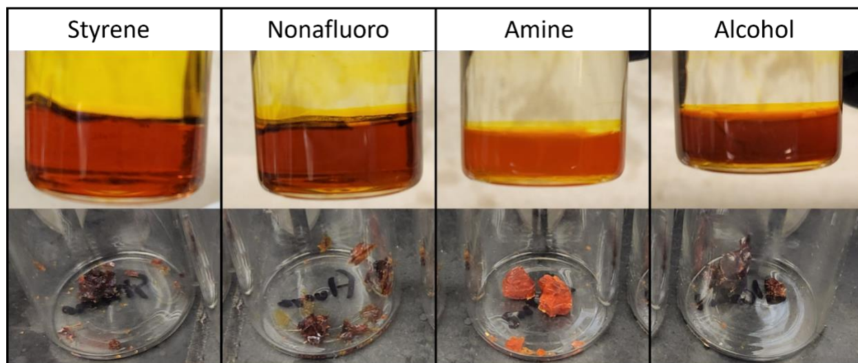
Figure 4. Images (20 mL scintillation vials) of the functionalized gels post-reaction (top) and after solvent exchange and drying (bottom). Styrene and nonafluoro utilized the in-situ method, while the amine and alcohol gel were post-functionalized. Each shows a visible difference in color, texture, and firmness.
