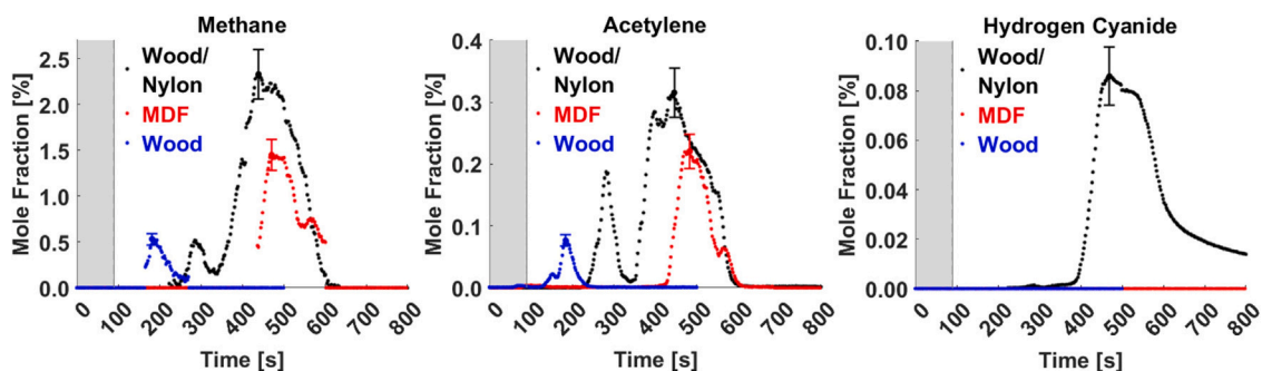
Fig. 9. Concentration profiles of \text{CH}_4 , \text{C}_2\text{H}_2 , and \text{HCN} in time for the three fuels. The uncertainty in the concentration measurements are shown by the error bars. The gray shaded region indicates when the propane burner was on.
