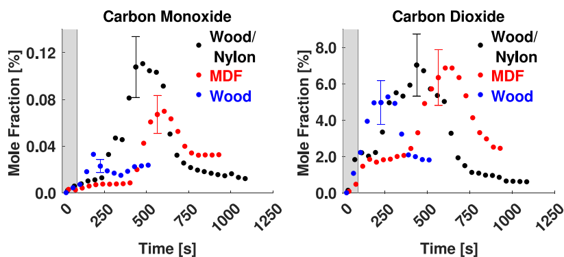
Fig. 3. Mole fraction measurements of CO and CO 2 in time for the varying fuels. The uncertainty in the concentration measurements are shown by the error bars. The gray shaded region indicates when the propane burner was on.
