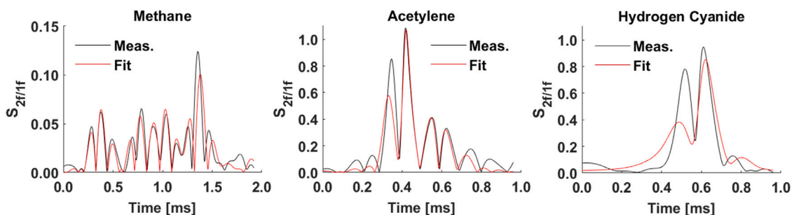
Fig. 8. Comparison of the 2f/1f measurement to the fitting routine output.
