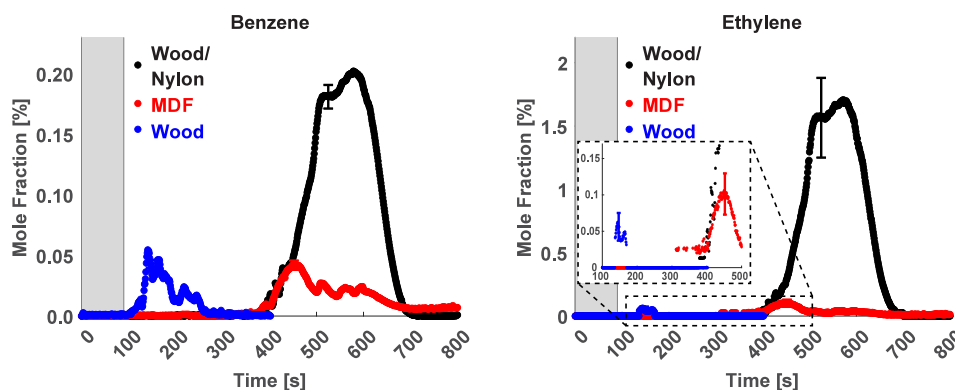
Fig. 6. Mole fraction measurements for C_6H_6 and C_2H_4 in time for the varying fuels. The uncertainty in the sensor is illustrated with a representative error bar for each species. The shaded region indicates when the time during which the propane burner was on.
