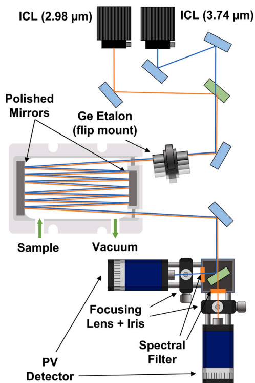
Fig. 7. Scanned-WMS optical setup deployed for HCN, CH_4 , and C_2H_2 .
