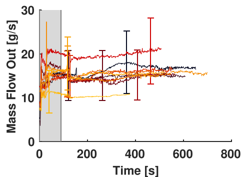
Fig. 11. All wood mass flow out measurements with error bars showing measurement uncertainty. The gray shaded region indicates when the propane burner was on.
