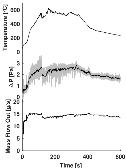
Fig. 10. Representative mass flow out experimental measurements and resulting mass flow out (bottom) for a wood crib experiment. The top plot shows the raw temperature measurements. And the middle plot includes the raw (gray) and smoothed (black) differential pressure measurements.
