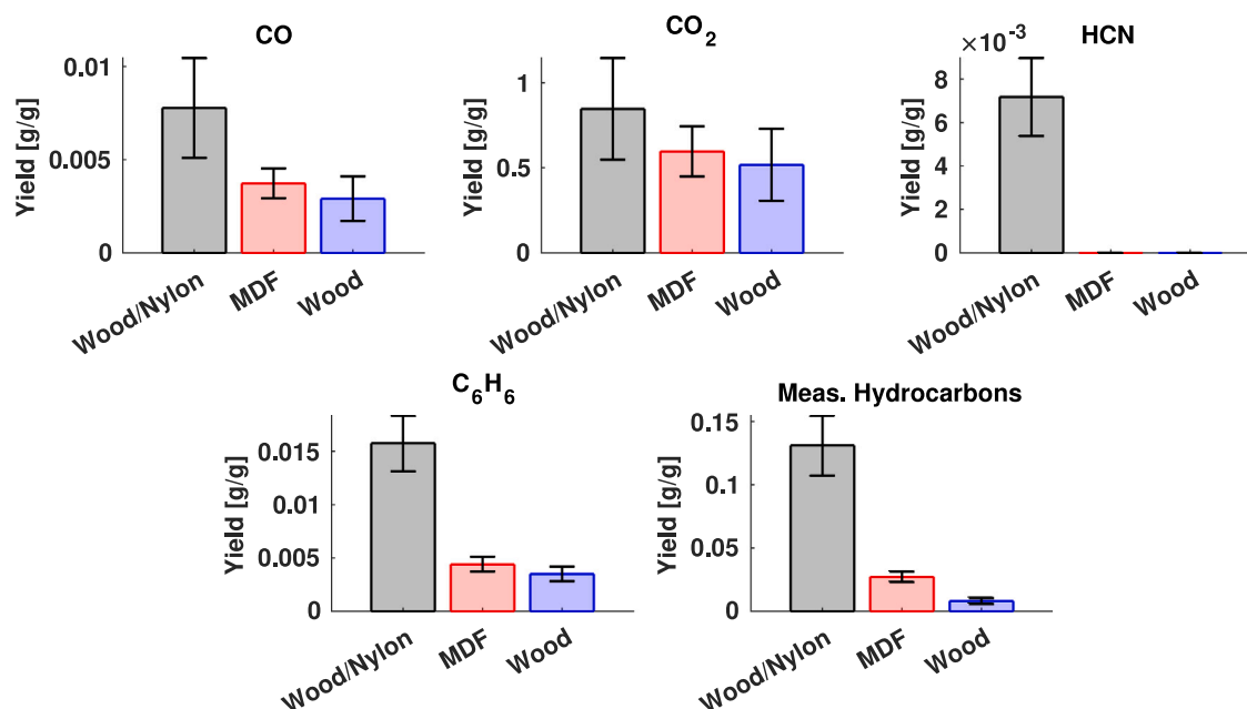
Fig. 12. Yields with the measurement uncertainty of CO, CO 2 , HCN, C 6 H 6 , and measured hydrocarbons from each fuel. The yield of measured hydrocarbons is the combined yield of C 6 H 6 , C 2 H 4 , C 2 H 2 , and CH 4 .
