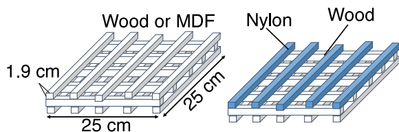
Fig. 2. Schematic of crib configurations Left : Single-fuel crib (wood or MDF), Right : Dual-fuel crib (wood and nylon).
