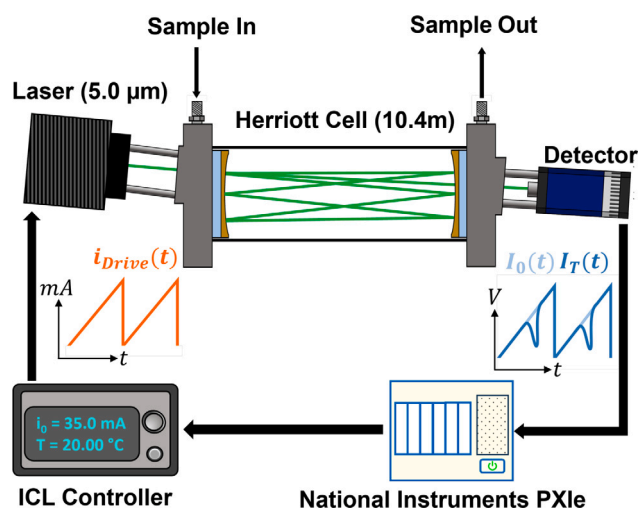
Fig. 4. Schematic of the LAS sensors for C 6 H 6 .
