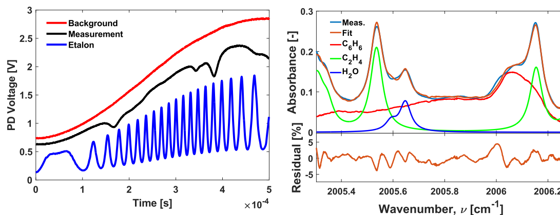
Fig. 5. Raw photodetector measurement for a representative wood/nylon fire and etalon measurement, which is used to develop a relationship between relative wavenumber and time, (left) and the associated post-processed absorbance spectra near 2006\text{ cm}^{-1} ( 4.98\text{ }\mu\text{m} ) showing the multi-spectral fit for benzene, water, and ethylene (right) [26,37].
