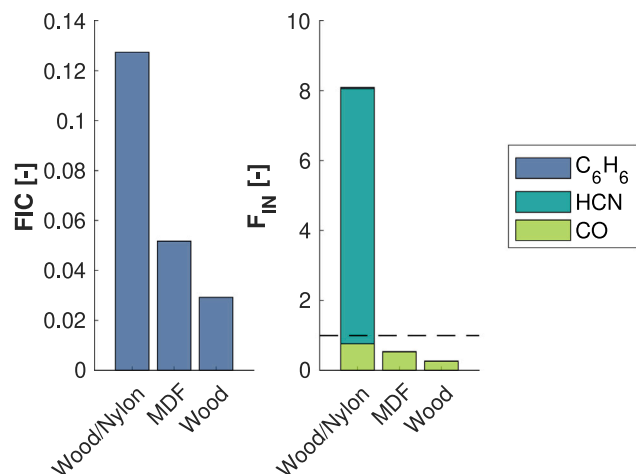
Fig. 13. Estimated fractional effective dose for incapacitation due to sensory irritants (left) and asphyxiation (right), if compartment combustion products are diluted at a 1:1 mass ratio of fresh air to fire effluents. This analysis considers the influence of CO, CO 2 , HCN, and C 6 H 6 concentration effects. The contribution of CO 2 is accounted for in F_{IN} as an effect on the ventilation rate. C 6 H 6 's contribution to F_{IN} for all fuels is small and cannot be visually seen.
