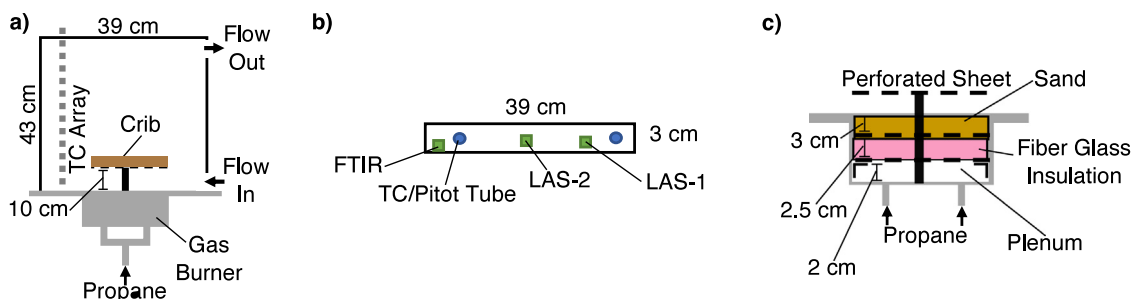
Fig. 1. Schematic of the experimental setup: (a) Side view, (b) Front view of upper slit with sensor measurement locations, (c) Detailed view of internal components of the gas burner configuration. The gas species that were measured at each sampling location were: CO and CO 2 for the FTIR; C 6 H 6 and C 2 H 4 for LAS-1; and C 2 H 2 , CH 4 , and HCN for LAS-2.
