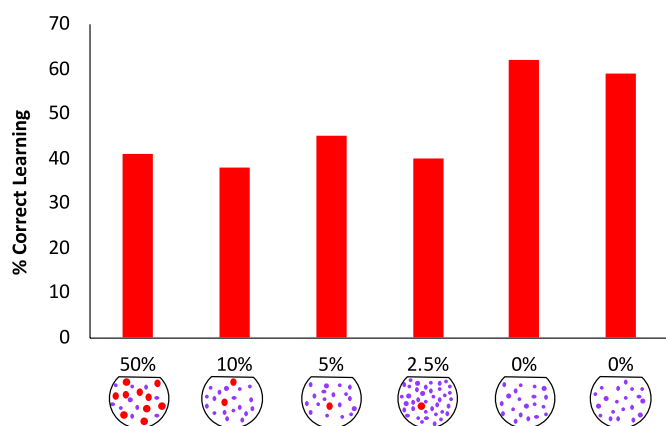
Fig. 1. Percent of children correctly identifying the Type B object when asked for the click in the Equi-Probable, Improbable, and Impossible conditions. X-axis indicates probability of drawing a Type B object across conditions.
