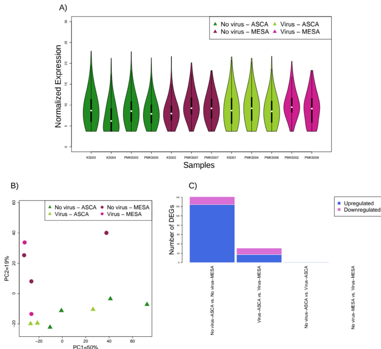
FIGURE 2 | Variation in gene expression across samples. (A) Violin plots show the distribution of normalised gene expression in all samples included in this study. The values from top to bottom represent the maximum, the upper quartile, the median, the lower quartile and the minimum in turn. The width of each violin represents the number of genes under the same expression. (B) Principal Component Analysis (PCA) based on normalised gene expression of all genes ( N = 11,214 ) included in this dataset. (C) Barplot showing the number of genes upregulated versus downregulated for the four comparisons included in the study. “No virus – ASCA” represents uninfected larvae fed with A. canadensis ; “Virus ASCA” represents infected larvae fed with A. canadensis ; “No virus – MESA” represents uninfected larvae fed with M. sativa ; “Virus – MESA” represents infected larvae fed with M. sativa . This labelling is followed in all figures and tables below.
