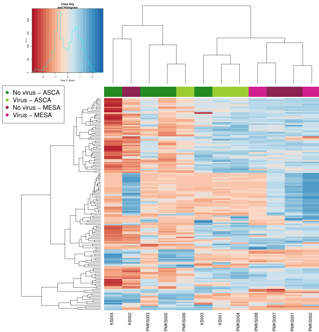
FIGURE 3 | Heatmap and hierarchical clustering of the top 150 differentially expressed genes between samples included in this study show that host plant treatment affects clustering of differentially expressed genes.
