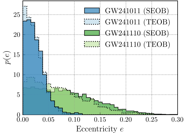
Figure 8. Posteriors on the orbital eccentricity of GW241011 and GW241110. Results are obtained using the SEOBNRv5EHM (Gamboa et al. 2025) and TEOBRESUMS-DALÍ (Nagar et al. 2024) waveform models, and eccentricities are quoted at a reference frequency of 13.33 Hz, when higher-order spherical harmonic modes first enter the observable frequency band. Neither event exhibits evidence for residual eccentricity. We bound e < 0.05 at 90% credibility for GW241011 under both waveform models. GW241110, meanwhile, yields 90% credible upper limits of e < 0.17 and e < 0.14 under the SEOBNRv5EHM and TEOBRESUMS-DALÍ models, respectively.
