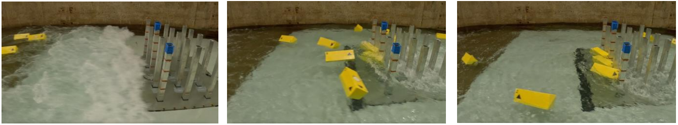
Figure 1. Experimental trial showing phases of debris damming: bore arrival (left), dam accumulation (center), and quasi-steady debris dam (right). Shown are the 3x5 column specimen configuration and 6.1m shipping containers debris.
