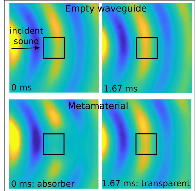
Figure 2. Time domain acoustic pressure measured in the empty waveguide (top) and with the time-modulated programmable metamaterial (bottom). The right pressure fields (transparent state) were measured 1.67 ms later than the left fields (absorber state), i.e. half the modulation period.
