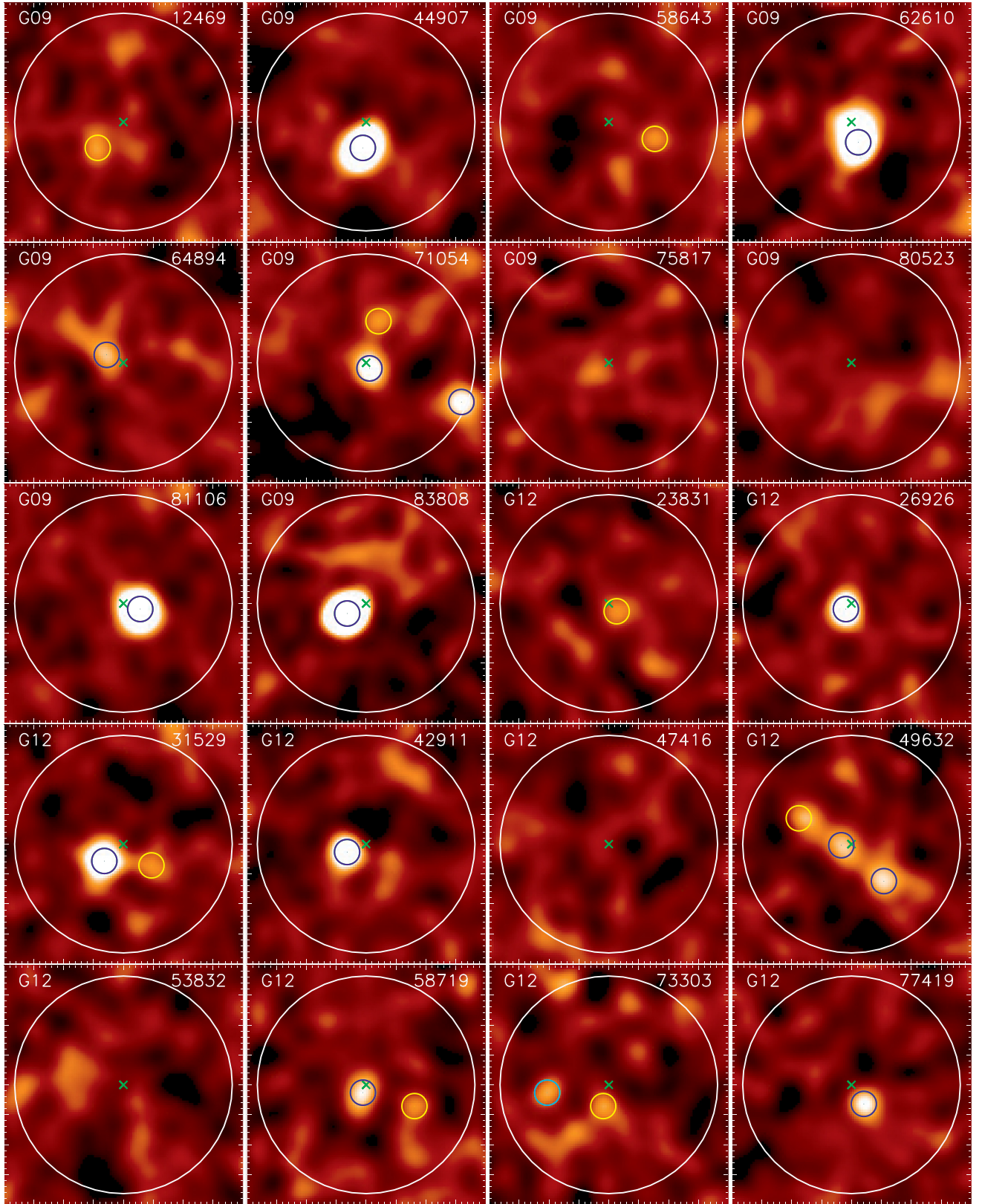
Figure A1. 80 \times 80 \text{ arcsec}^2 postage stamps of the 93 H-ATLAS targets included in our analysis. Images correspond to the 1.1 mm AzTEC SNR maps. Green crosses and white circles indicate the H-ATLAS targeted position and the adopted search radius (36.6 arcsec), respectively. Small circles (9.5 arcsec in diameter) mark the position of AzTEC detections, with: yellow corresponding to 3.0 \leq \text{SNR} < 3.5 , light blue to 3.5 \leq \text{SNR} < 4.0 , and dark-blue to \text{SNR} \geq 4.0 .
