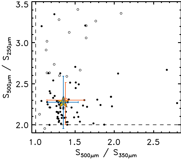
Figure 1. Colour selection ( S_{500 \mu\text{m}}/S_{250 \mu\text{m}} > 2 and S_{500 \mu\text{m}}/S_{350 \mu\text{m}} > 1 ) of the H-ATLAS targets observed with AzTEC: filled black circles identified in the 250 \mu\text{m} map and empty circles in the 350 \mu\text{m} (i.e. BANDFLAG 1 and 2 in Ivison et al. (2016), respectively). All targets were detected above 5\sigma at 500 \mu\text{m} . The yellow star indicates the average colour of the sample, while the blue and orange circles indicate, respectively, the median colour of the targets with and without AzTEC detections above a 4\sigma level. The similar colours shown by the two sub-samples suggest that differences in SEDs cannot explain the bulk of AzTEC non-detections discussed in Section 3.2.
