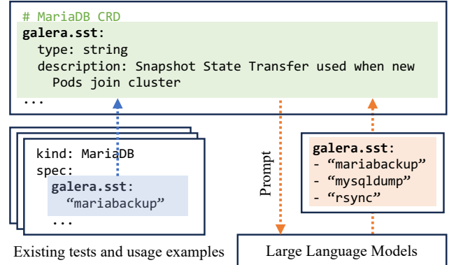
Figure 5: Synthesizing values for the galera.sst property using existing tests and usage examples, and LLMs.
