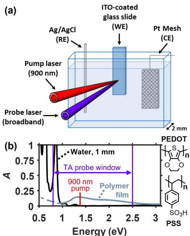
Figure 1. (a) Spectroelectrochemistry cell for electrochemical doping of conducting polymers in aqueous electrolyte designed for steady-state and ultrafast transient absorption spectroscopy in the visible/near-infrared region. (b) Absorption spectrum of a 1 mm layer of water compared to that of a doped PEDOT:PSS film on ITO/glass held at -0.2 V (vs Ag/AgCl), highlighting the pump and probe wavelengths used in the TA measurements. The 900 nm pump wavelength is selected because it can excite the polaronic transition in the polymer without exciting a vibrational transition in the water. Immeasurable parts of the spectrum due to intense water absorption were removed.
