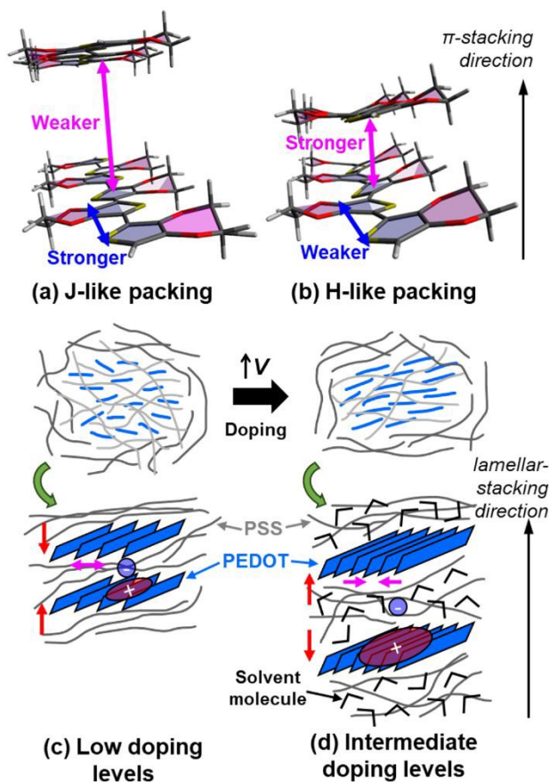
Figure 7. Illustration of the doping-induced changes in (a,b) PEDOT aggregation behavior and (c,d) PEDOT:PSS film nanostructure. In J-like aggregates (a), the PEDOT chains are more planar and have stronger intrachain coupling. The interchain coupling is weak and the chains are more isolated. In H-aggregates (b), the PEDOT chains are more twisted and can thus more tightly \pi -stack, increasing interchain coupling and decreasing intrachain coupling. At low doping levels (c), the lamellae are more compressed and the PEDOT chains are more separated like in J-aggregates with localized polarons. At intermediate doping levels (d), the lamellae expand with solvent from the electrolyte and the PEDOT chains pack more tightly like in H-aggregates with more delocalized polarons.
