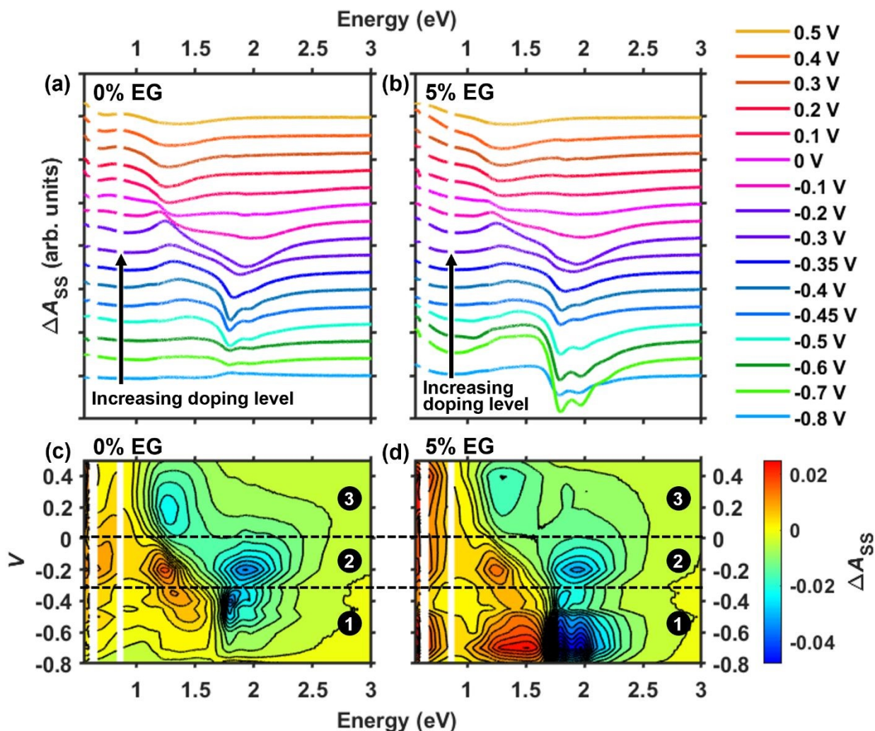
Figure 3. (a,b) Absorbance difference ( \Delta A_{SS} ) traces for the PEDOT:PSS films cast using 0% and 5% ethylene glycol (EG) cosolvent. The spectra, which are offset for clarity, were calculated by taking the difference in the absorption spectra with respect to each step in voltage (vs Ag/AgCl). (c,d) Contour plots of the absorbance difference data in (a) and (b) using 25 evenly spaced lines, where negative changes are in blue and positive changes are in red.
