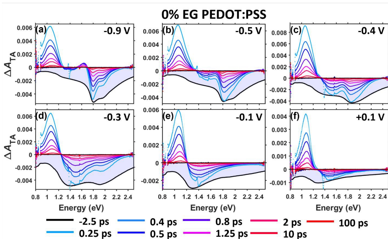
Figure 4. TA-SEC measurements of the pristine PEDOT:PSS film in 0.5 M KCl electrolyte in the visible and near-IR spectral regions as a function of applied voltage (vs Ag/AgCl). The voltages used were (a) -0.9 V, (b) -0.5 V, (c) -0.4 V, (d) -0.3 V, (e) -0.1 V, and (f) +0.1 V, and the excitation energy was 1.37 eV (900 nm). Prior to each measurement, the film was allowed to equilibrate under bias for 120 seconds. The associated ground state
