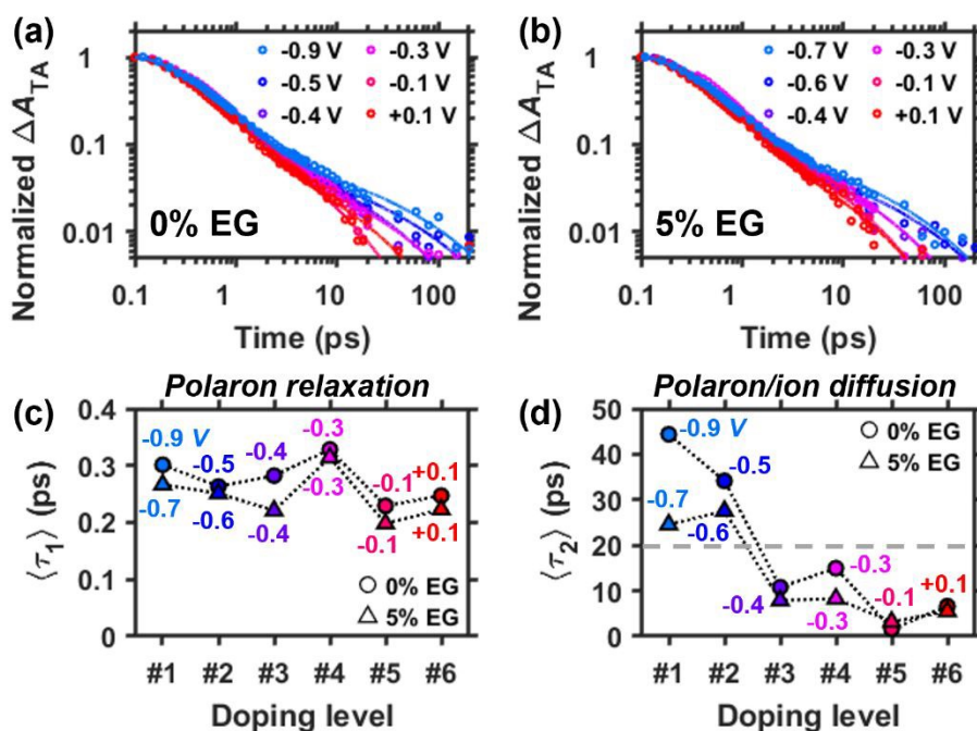
Figure 6. Voltage-dependent (vs Ag/AgCl), normalized TA kinetics selected at the PIA peak maximum and averaged over 1.05 – 1.09 eV for the (a) 0% and (b) 5% EG samples. Data are displayed as markers, while the solid lines are fits to a sum of two stretched
