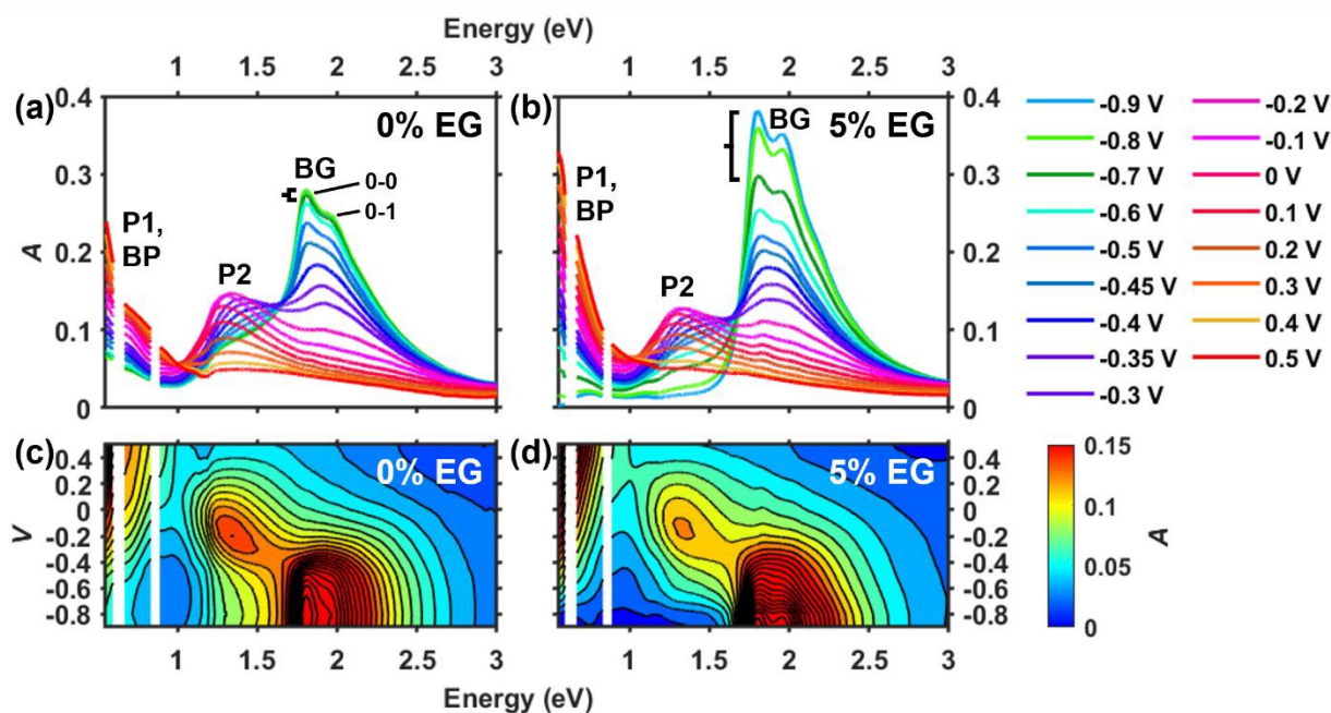
Figure 2. (a,b) Voltage-dependent absorption spectra of 0% EG and 5% EG PEDOT:PSS films in 0.5 M KCl. Each voltage (vs Ag/AgCl) was applied for 120 s to equilibrate the film prior to recording the absorbance. The black brackets point out changes in the bandgap absorption signal when voltage is changed from -0.7 to -0.9 V. (c,d) Contour plots of the absorbance data in (a) and (b) using 25 evenly spaced lines.
