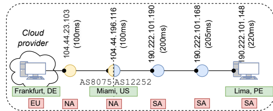
Fig. 5. Illustrative traceroute
