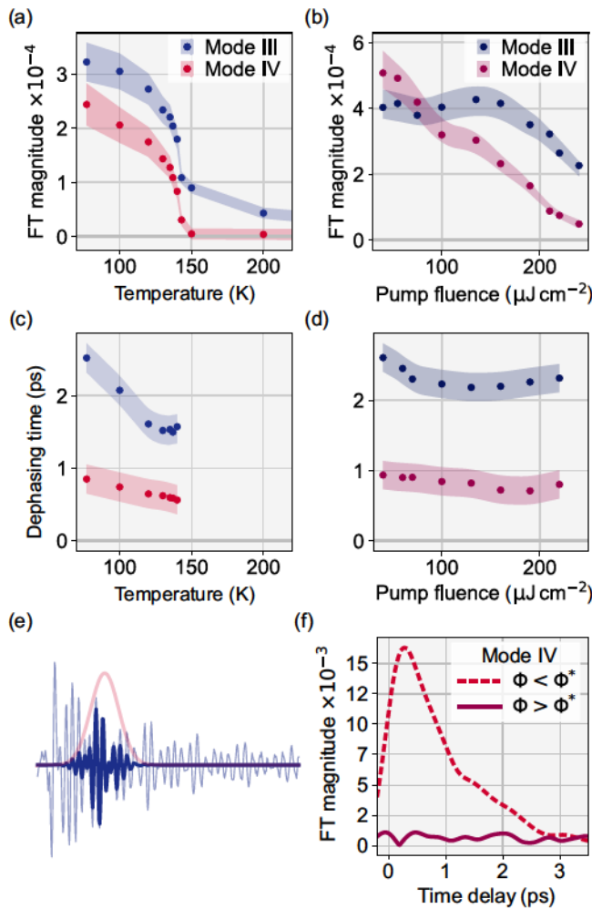
FIG. 5. Parameters of Modes III and IV, shown in blue and red, respectively. (a) Temperature and (b) fluence dependence of FT magnitudes, normalized to corresponding pump-fluence values. (c) Temperature and (d) fluence dependence of phonon dephasing time, determined by STFT analysis. The error bars are represented by the thickness of the filled areas. (e) Illustration of the STFT: sliding Gaussian time window \mathcal{G}(\sigma, \mu) selects data range within which the mode content is explored. (f) STFT of Mode IV below ( \Phi = 0.12 \Phi^* ) and above ( \Phi = 3.3 \Phi^* ) threshold fluence ( T = 77 K), showing that Mode IV is not present for \Phi > \Phi^* .
