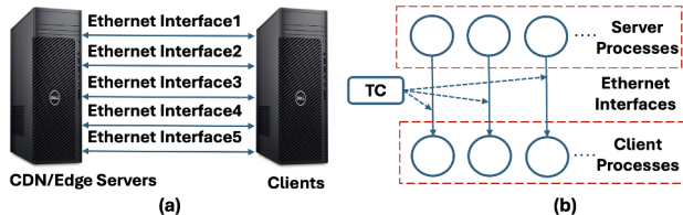
Fig. 6. (a): Client and server processes are on two separate machines. (b): Linux TC controls bandwidth, delay, and loss for each path.
