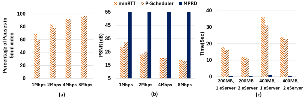
Fig. 8. (a): Percentage of pauses for Big Buck Bunny video. (b): PSNR. (c) File download time.
