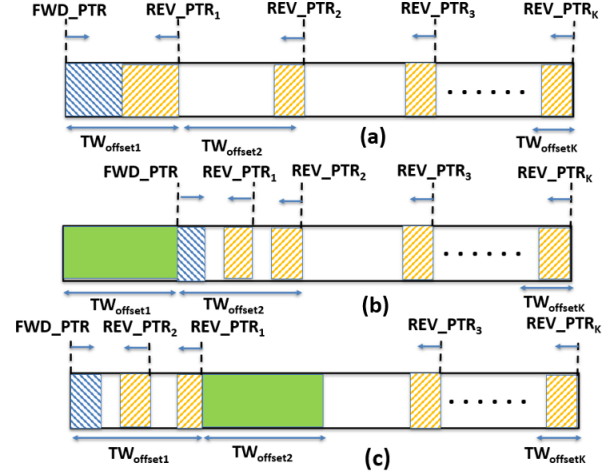
Fig. 5. (a): Initial placement of forward and reverse pointers at the client reception window. The dashed parts represent the segments transmitted by the associated server. (b): When forward and reverse pointer 1 cross over (i.e., finish transmitting the segments between them), MPRD reassigns them to help with transmitting segments in TW_{offset2} . The green blocks shows the segments received by the client. (c): As reverse pointer 2 finishes transmitting its segments, MPRD reassigns it to be in between the forward pointer and reverse pointer 1.
