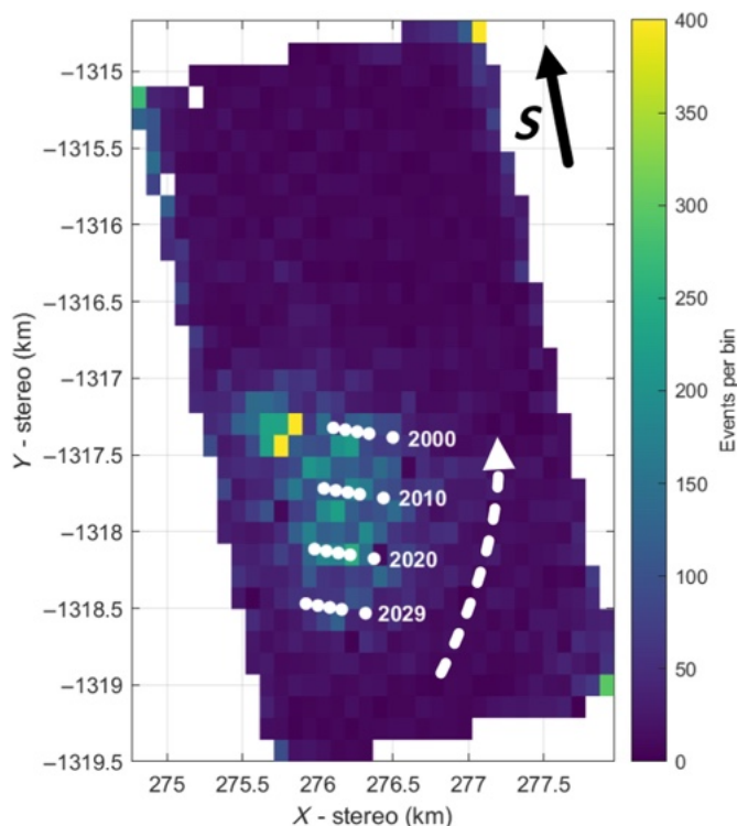
Figure 10. Event density for 1 day of data, 24 January 2023, clustered into 100 × 150 m bins. Approximately 26,000 seismic events were detected for the 24 hr period. The dashed arrow indicates ice flow direction. There is a high density of events in the shear margin southeast of the array. The color version of this figure is available only in the electronic edition.
