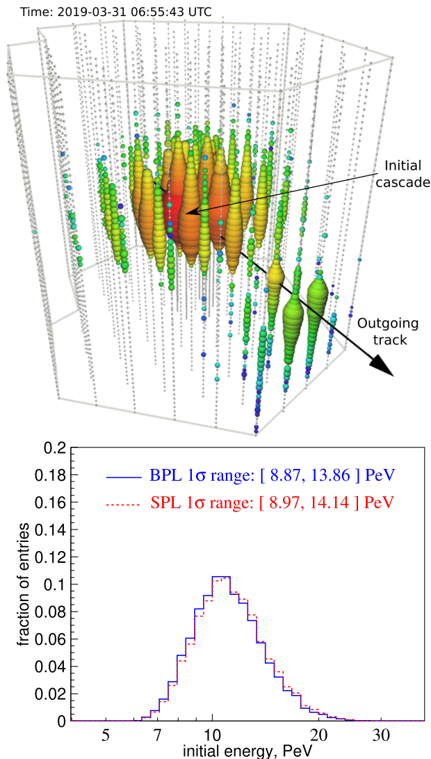
FIG. 14. IceCube’s highest energy neutrino event: An event view of the highest neutrino energy event recorded to date by IceCube is shown (top). The size of the spheres indicates the number of photoelectrons recorded by the respective DOMs. The earliest deposits are shown in red, with later deposits depicted first in yellow, then green, with the last deposits in blue. The duration of the event is 22596 ns. This event stands out as an exceptional instance of a starting track, where the initial muon-neutrino interaction occurs inside the detector, creating a cascade feature, and the outgoing muon lepton leaves a track signature in the detector volume. The cascade and track portions of the event are highlighted. The reconstructed neutrino energy distribution of the highest neutrino energy event recorded to date during IceCube’s data taking is shown (bottom). The distribution is derived from multiple simulations of the neutrino interaction that could have occurred to produce the observed event. The median neutrino energy is 11.4 PeV, assuming the best-fit broken power-law spectral model for the astrophysical neutrino flux.
